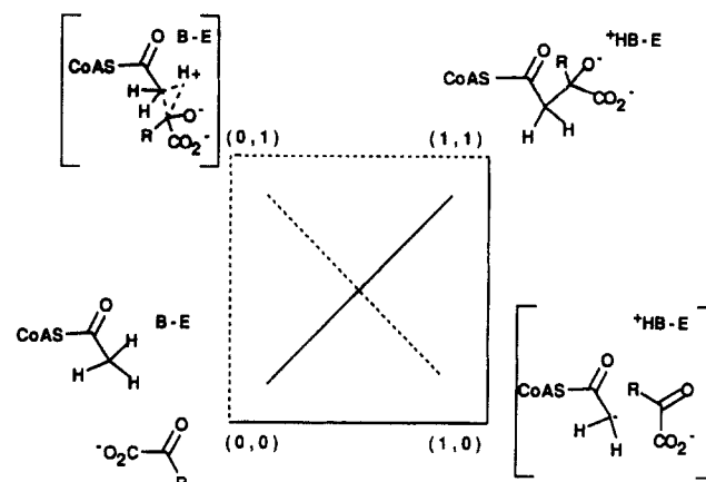
SCHEME 11. Grunwald Disparity Diagram for Malate Synthase
