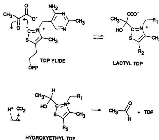
SCHEME 25. Mechanism of Thiamin-Catalyzed Decarboxylation of Pyruvate
