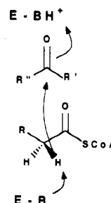
SCHEME 10. Reaction Diagram for Claisen Enzymes
