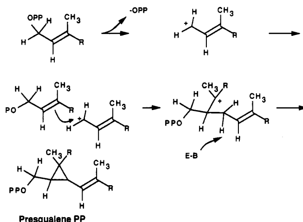
SCHEME 2. Formation of Presqualene PP from Farnesyl PP
